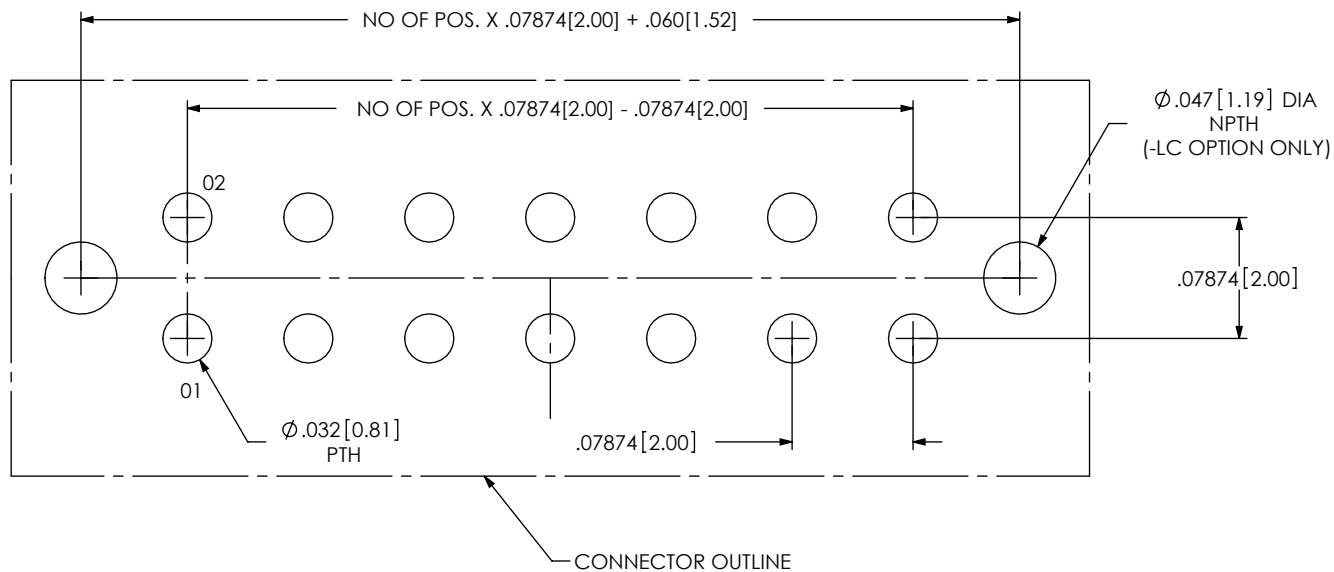
FIGURE 1 LTMM-107-XX-XX-D-LC-XX
