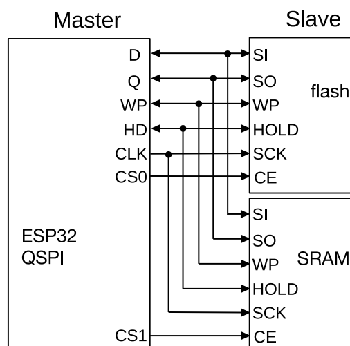
Figure 19: Parallel QSPI
