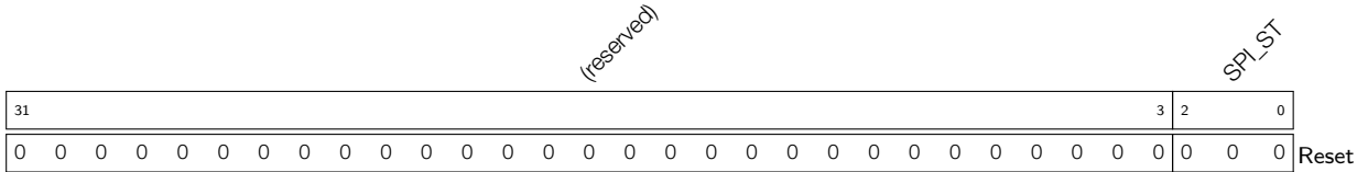
Register 7.24: SPI_EXT2_REG (0xF8)
