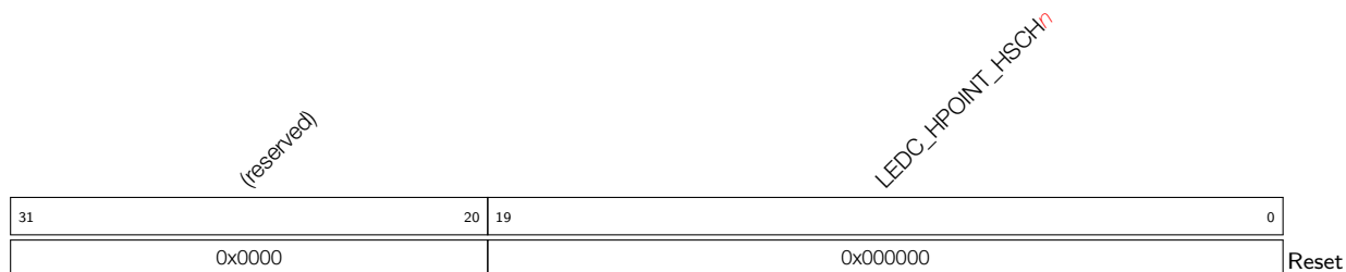
Register 14.2: LEDC_HSCH n _HPOINT_REG ( n : 0-7) (0x20+0x10* n )
