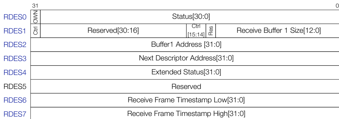
Figure 47: Receive Descriptor
