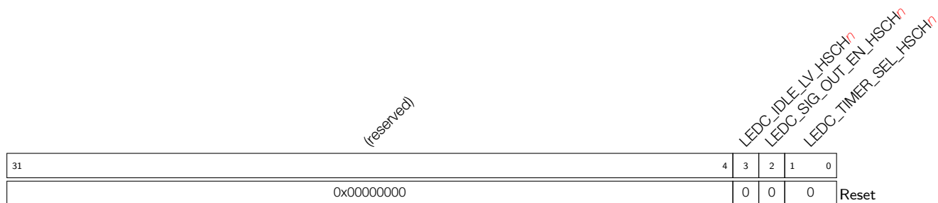
Register 14.1: LEDC_HSCH n _CONF0_REG ( n : 0-7) (0x1C+0x10* n )
