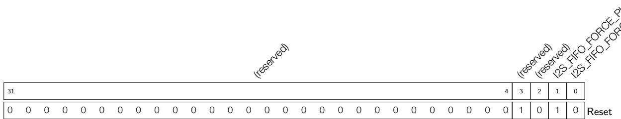
Register 12.29: I2S_PD_CONF_REG (0x00a4)
