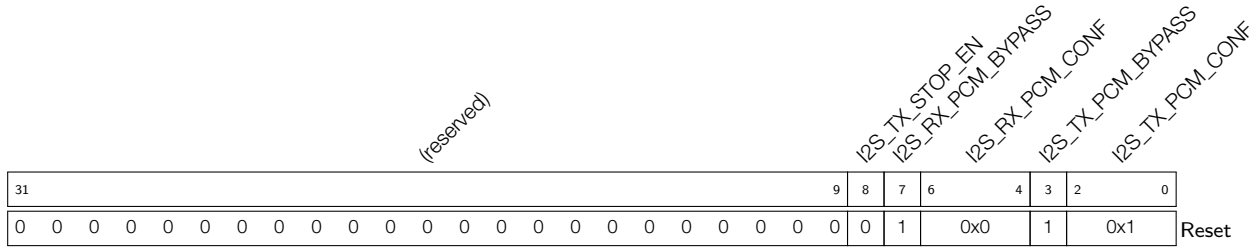
Register 12.28: I2S_CONF1_REG (0x00a0)
