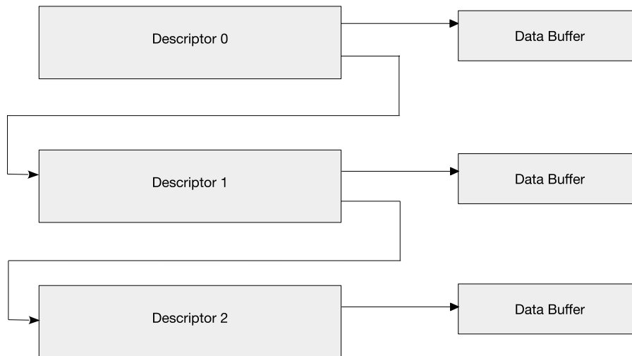
Figure 37: Descriptor Chain
