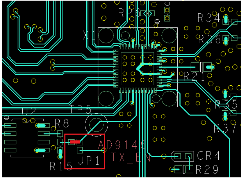
Figure 6: TX Enable to DPG Jumper Configuration
