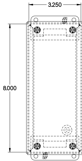
FRONT VIEW
