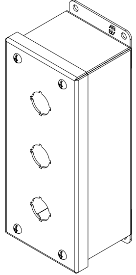
ISOMETRIC VIEW
