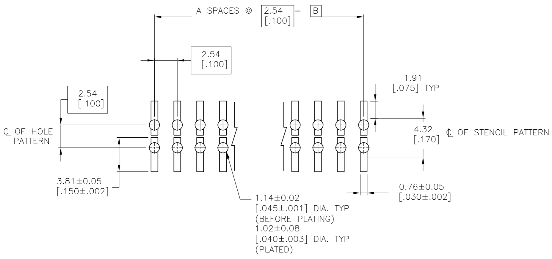
RECOMMENDED PC BOARD MOUNTING DIMENSIONS FOR 1.60[.063] THICK PC BOARD AND 0.305[.0120] STENCIL THICK
