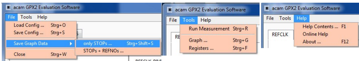
Figure 5: Menu selections
