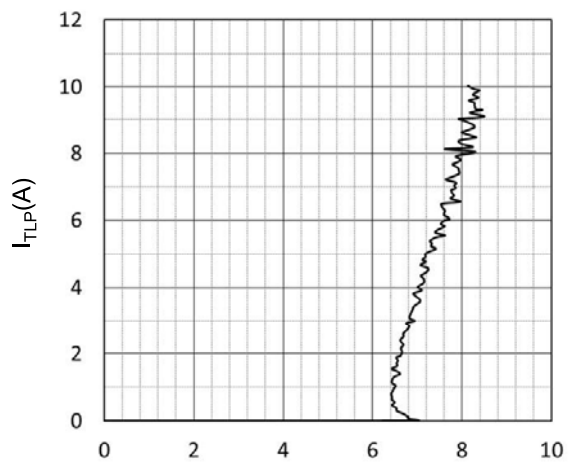
TRANSMISSION LINE PULSE
