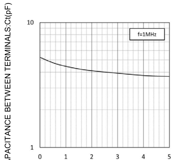
REVERSE VOLTAGE:VR(V) VR-Ct CHARACTERISTICS
