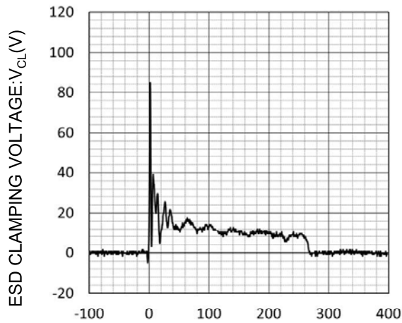
TIME(ns) ESD CLAMPING VOLTAGE (IEC61000-4-2 +8kV CONTACT)
