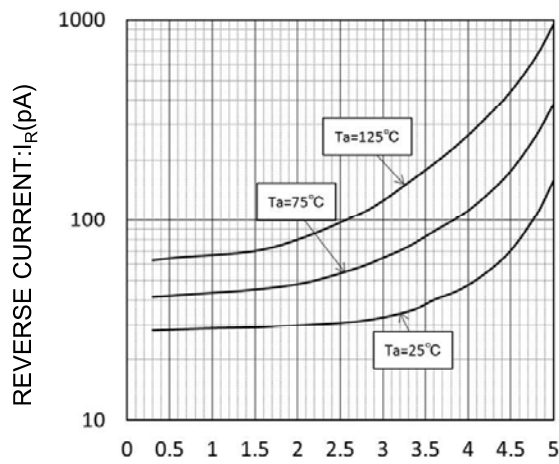
REVERSE VOLTAGE:VR(V) VR-IR CHARACTERISTICS
