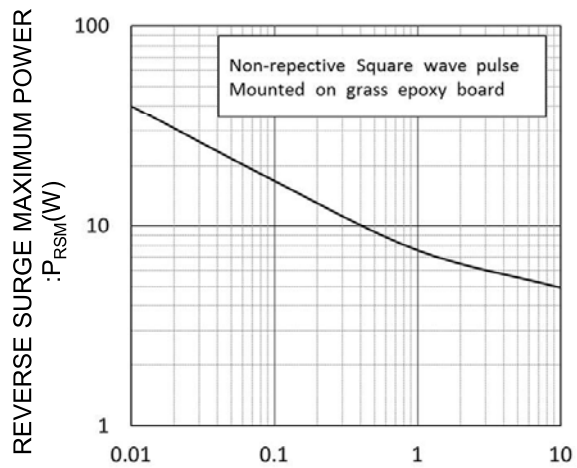
PULSE TIME CHARACTERISTICS
