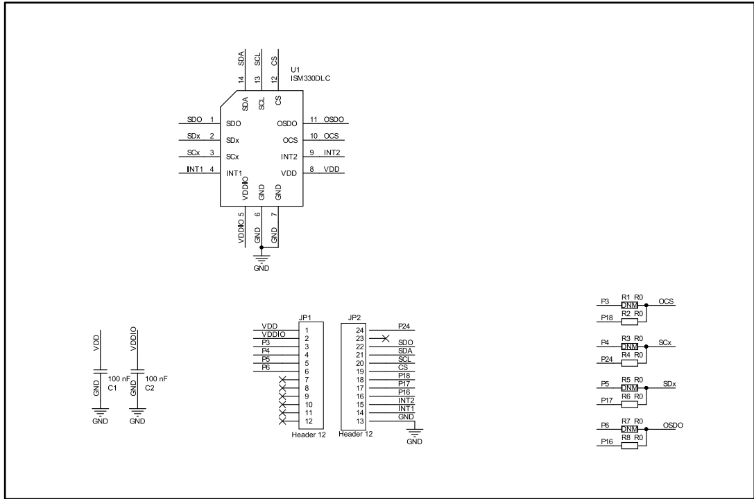
Figure 1: STEVAL-MKI182V1 circuit schematic
