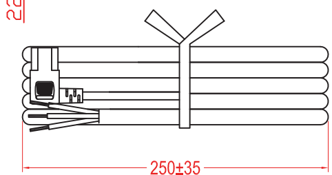
Hank dimension
