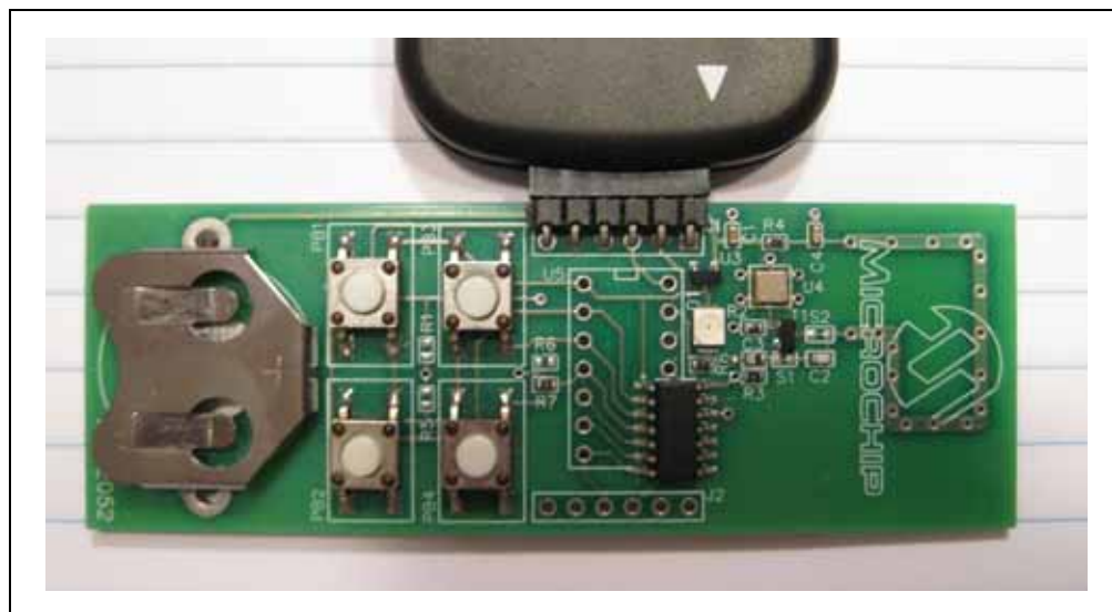
FIGURE 1-3: TRANSMITTER BOARD
