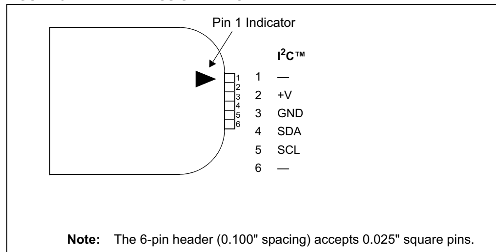
FIGURE 5-1: PIN ASSIGNMENTS
