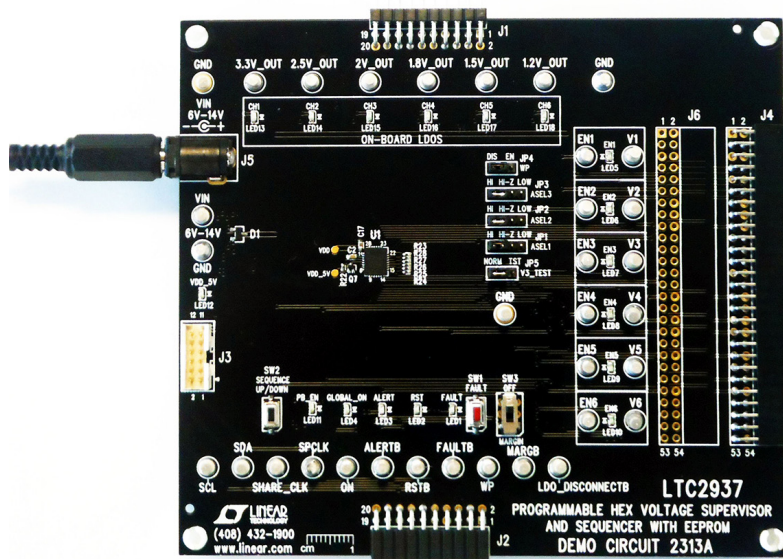
Figure 3. DC2313A Standalone
