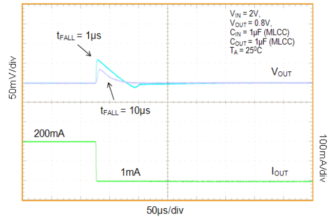
Figure 50. Load Transient Response - Falling Edge, I_{OUT} = 1\text{ mA} - 200\text{ mA} , C_{OUT} = 1.0\text{ }\mu\text{F}
