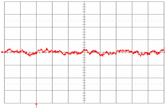
Fig. 25: Input reflected ripple current, i_s (10 mA/div.), measured through 10 \mu\text{H} at the source at full rated load current and V_{in} = 48 \text{ V} . Refer to Fig. 23 for test setup. Time scale: 1 \mu\text{s}/\text{div} .
