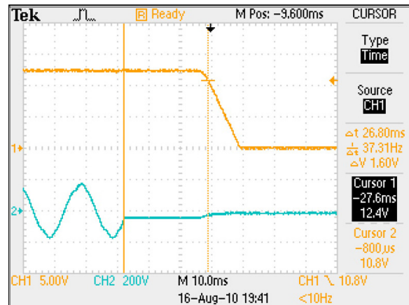
Figure 9: LCB150E Hold-up Time Vin = 115Vac Load: Io = 12.5A Ch 1: Vo Ch 2: AC Mains
