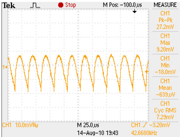
Figure 7: LCB150E Ripple and Noise Vin = 230Vac Load: Io = 12.5A Ch 1: Vo
