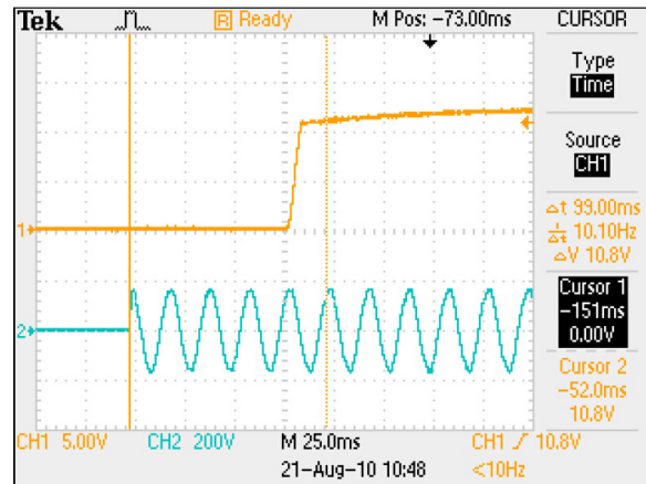
Figure 8: LCB150E Turn On Delay Vin = 115Vac Load: Io = 12.5A Ta = 25 °C Ch1: Vo Ch2: Vin
