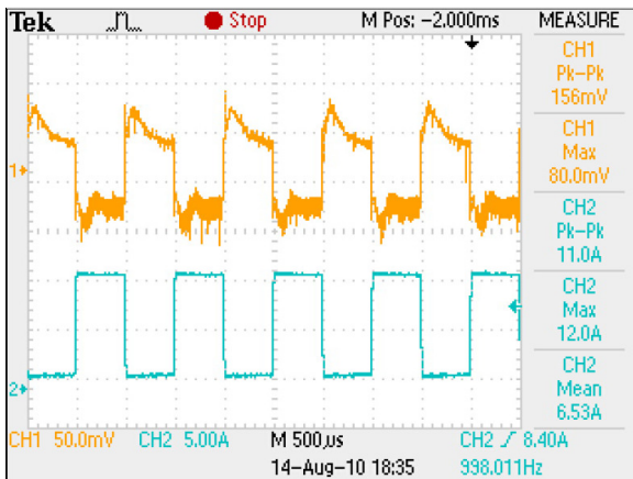
Figure 11: LCB150E Transient Response Vin = 230Vac Load: Io = 10% to 90% load change Ch 1: Vo Ch 2: Io
