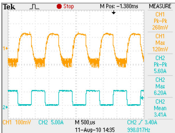
Figure 23: LCB150N Transient Response Vin = 230Vac Load: Io = 10% to 90% load change Ch 1: Vo Ch 2: Io
