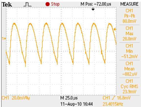
Figure 19: LCB150N Ripple and Noise Vin = 230Vac Load: Io = 6.5A Ch 1: Vo
