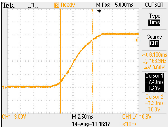
Figure 10: LCB150E Rise time Vin = 230Vac Load: Io = 12.5A Ch1: Vo
