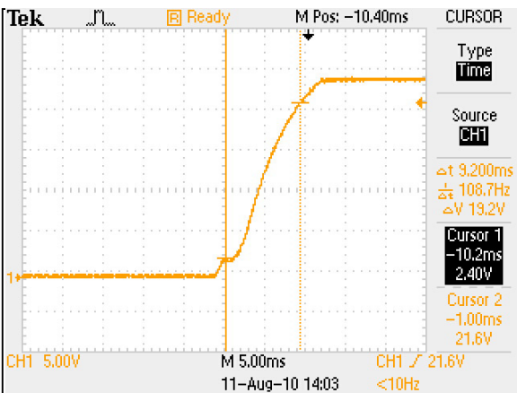
Figure 22: LCB150N Rise time Vin = 115Vac Load: Io = 6.5A Ch1: Vo
