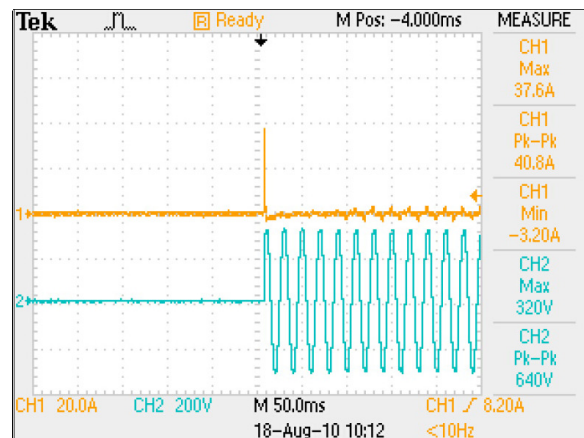
Figure 6: LCB150D Inrush Current Vin = 264Vac Load: Io = 18A Turn on Angle = 90 deg Ch 1: Io Ch 2: AC Mains
