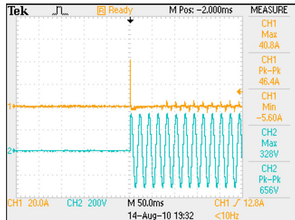
Figure 12: LCB150E Inrush Current Vin = 264Vac Load: Io = 12.5A Turn on Angle = 90 deg Ch 1: Iin Ch 2: AC Mains
