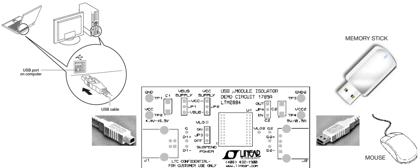
Figure 2. Demo Board Setup
