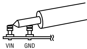
Figure 2. Proper Scope Probe Positioning for Output Ripple Measurement
