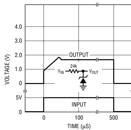
Response Time
