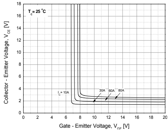
Fig. 4 Saturation voltage vs. gate bias
