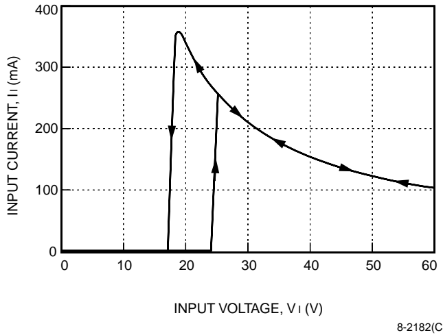
Figure 2. ME005B Typical Input Characteristics with I_o = I_{o, max} and T_A = 25\text{ }^\circ\text{C} (Arrows Indicate Hysteresis)
