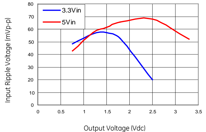
Figure 27. Input ripple voltage for various output with 1 \times 150 \mu F polymer and 1 \times 47 \mu F ceramic capacitors at the input (full load)
