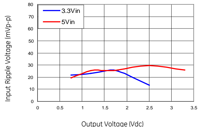
Figure 28. Input ripple voltage for various output with 3 \times 150 \mu F polymer and 2 \times 47 \mu F ceramic capacitors at the input (full load)
