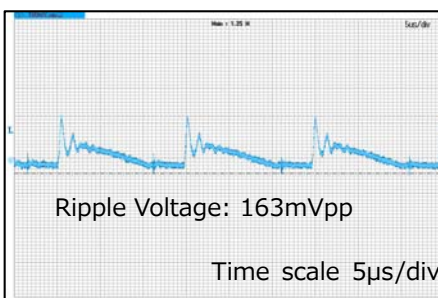
V_{IN}=230Vac, I_{OUT}=1.0A
