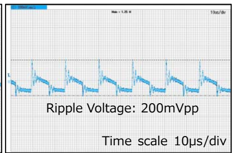
V_{IN}=100Vac, I_{OUT}=1.25A
