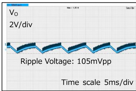
V_{IN}=100Vac, I_{OUT}=20mA
