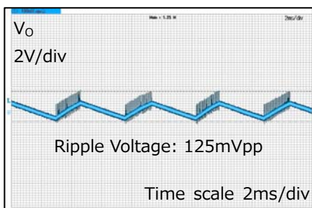
V_{IN}=230Vac, I_{OUT}=20mA
