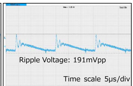
V_{IN}=230Vac, I_{OUT}=1.25A
