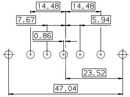
LAYOUT DIMENSIONS (after plating) CONNECTOR SIDE VIEW
