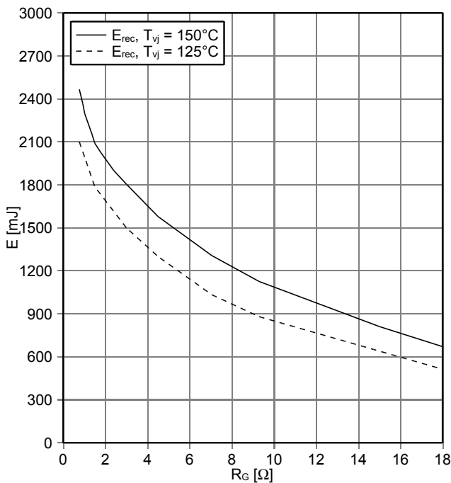
Schaltverluste Diode, Brems-Chopper (typisch) switching losses Diode, Brake-Chopper (typical) E_{rec} = f(R_G) I_F = 1000 A, V_{CE} = 1800 V
