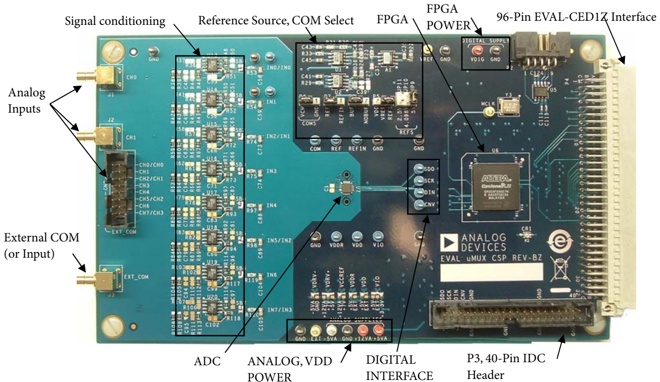
Figure 1. Evaluation Board
