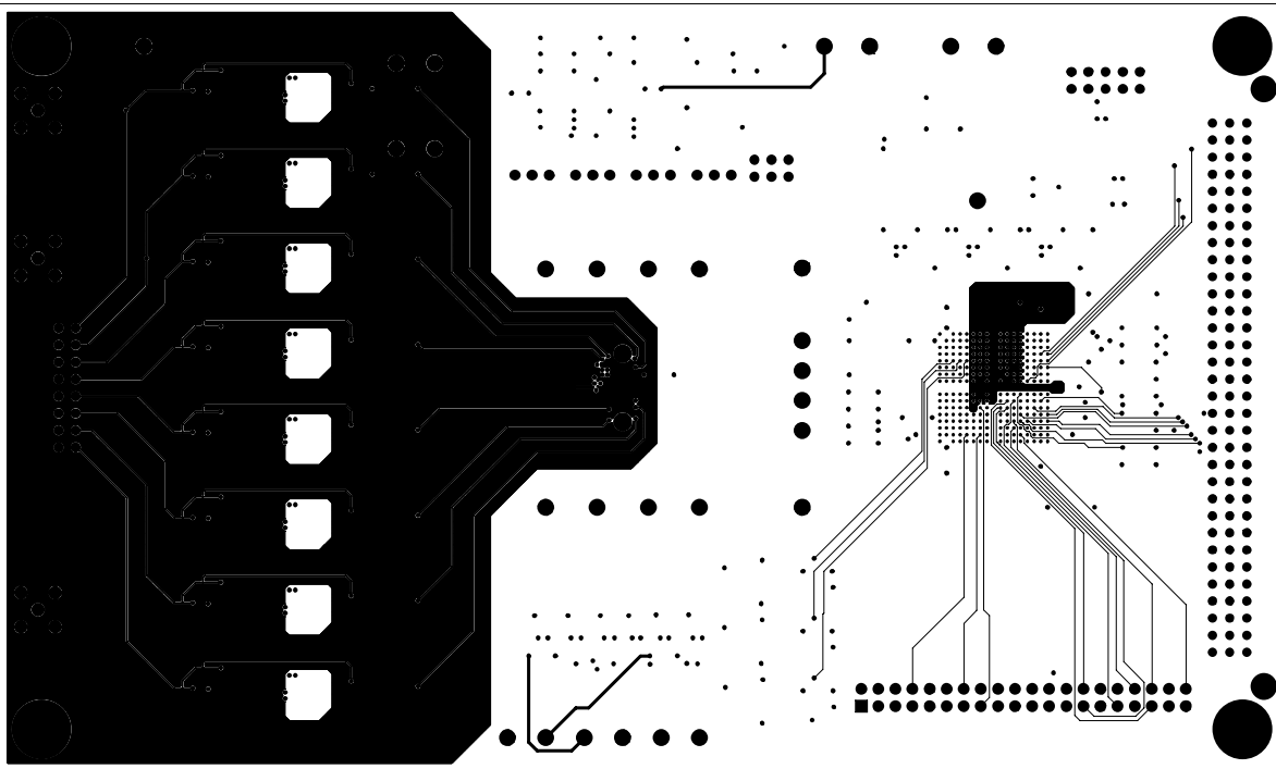
Figure 21. Inner Layer 1 (Viewed from top side)
