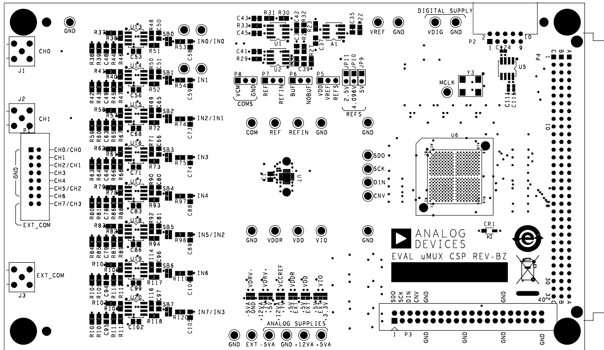
Figure 20. Top Side Silk-Screen (Viewed from top side)
