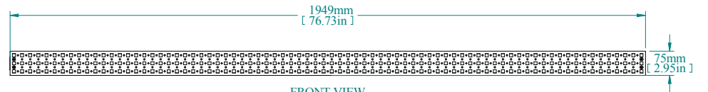
FRONT VIEW
