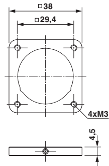
Dimensional drawing
