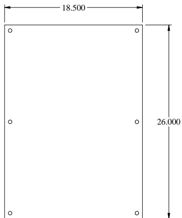
INNER PANEL
