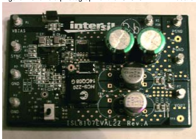
FIGURE 1. ISL8107EVAL2Z
