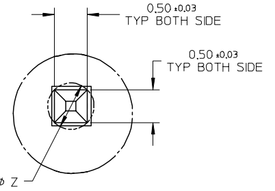
DETAIL Z
