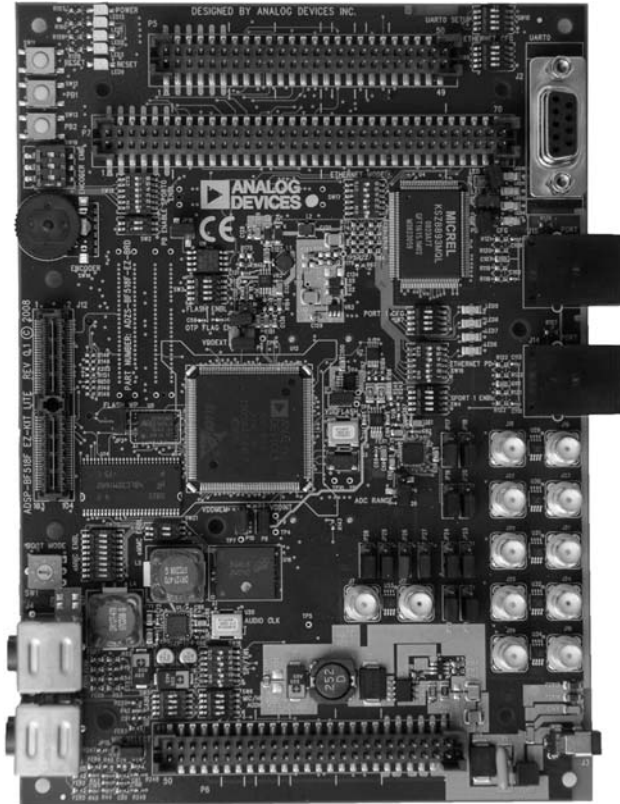
Figure 2-4. ADSP-BF518F EZ-KIT Lite Evaluation System
