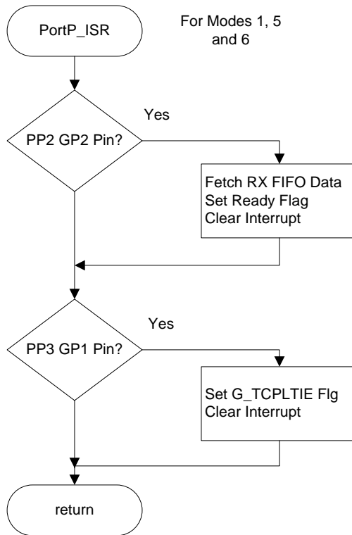
Receiver Mode 1 Flow Chart
