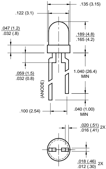
HLMP-K150/K155
