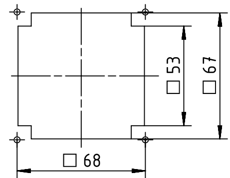
panel cut out (1:2)
