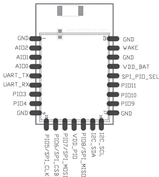
Figure 1. Pinout (Topview)
