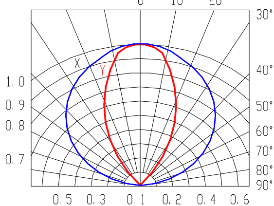
Radiation Characteristics
