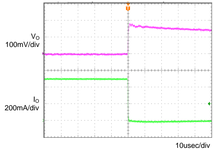
Figure 6. Transient Response (0.5→0A) C o =1μF, T a =-40°C
