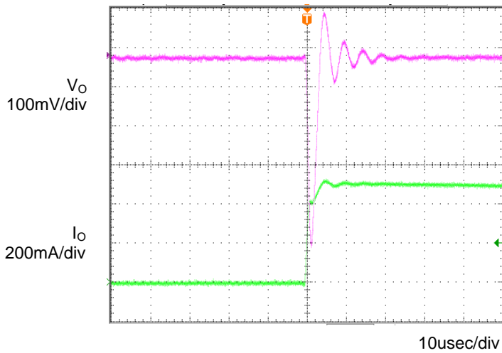
Figure 5. Transient Response (0→0.5A) C o =1μF, T a =105°C
