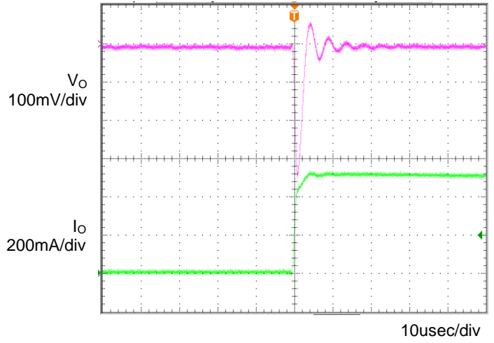
Figure 4. Transient Response (0→0.5A) C o =1μF, T a =25°C
