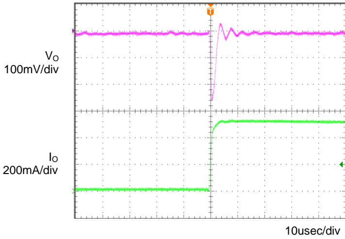
Figure 3. Transient Response (0→0.5A) C o =1μF, T a =-40°C
