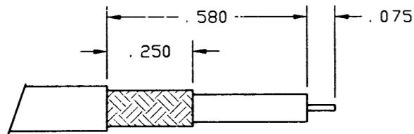
CABLE STRIPPING DIMENSIONS
