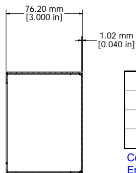
SECTION RR-RR
