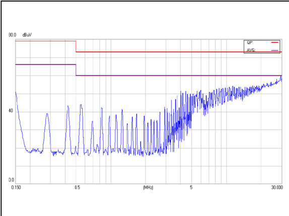
Figure 55: ASA01BB24-M Conduction Emission of EN55022 Class A Vin = 24Vdc Load: Io = ± 0.25A
