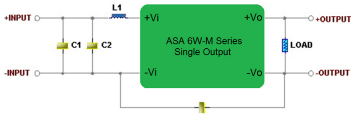
Single Output
