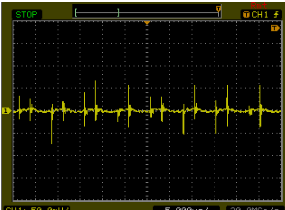
Figure 67: ASA01A48-M Ripple and Noise Measurement Vin = 48Vdc Load: Io = 1A Ch 1: Vo
