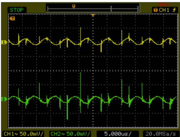
Figure 83: ASA01BB48-M Ripple and Noise Measurement Vin = 48Vdc Load: Io = ± 0.25A Ch 1: Vout1 Ch 2: Vout2
