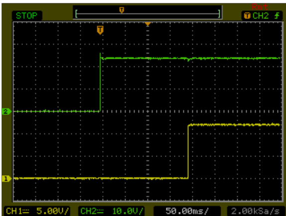
Figure 53: ASA01BB24-M Output Voltage Startup Characteristic by Vin Vin = 24Vdc Load: Io = ± 0.25A Ch1: Vin Ch2: Vo
