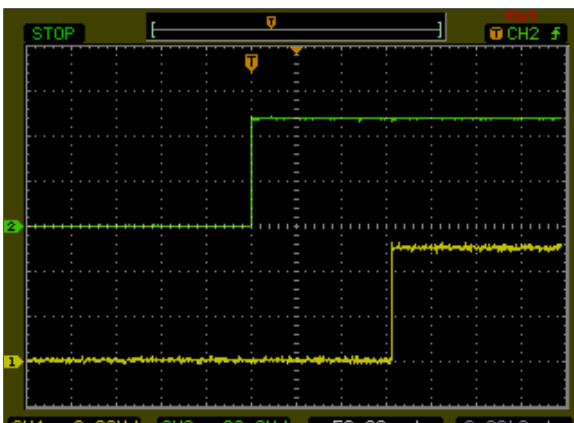
Figure 69: ASA01A48-M Output Voltage Startup Characteristic by Vin Vin = 48Vdc Load: Io = 1A Ch1: Vin Ch2: Vo
