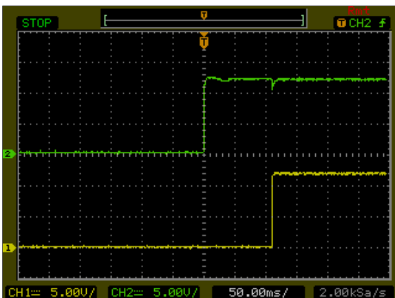
Figure 13: ASA001B12-M Output Voltage Startup Characteristic by Vin Vin = 12Vdc Load: Io = 0.5A Ch1: Vin Ch2: Vo
