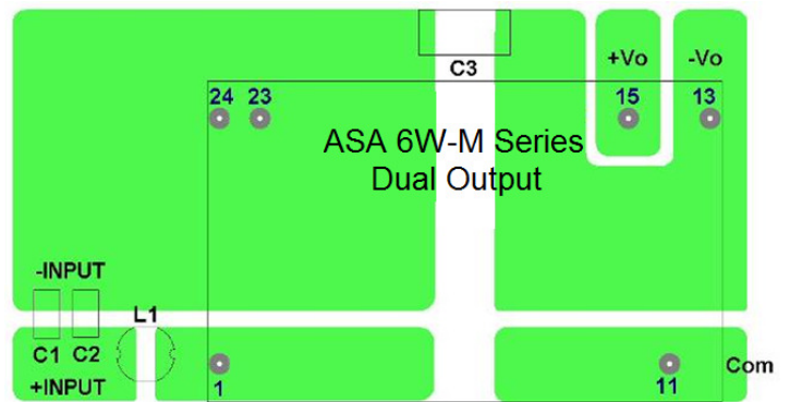
Dual Output
