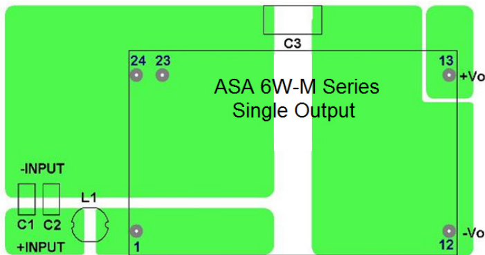
Single Output
